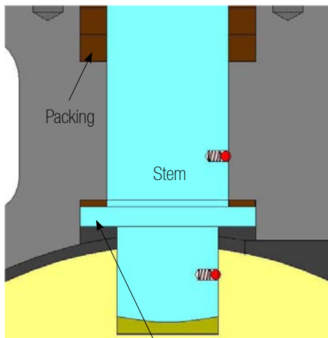
Blow Out Proof Stem
