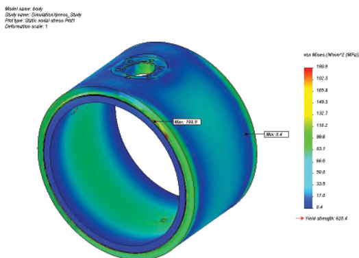
Body – 20" Class 600 – Fully Welded Type
