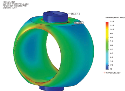
Ball – 20" Class 600 – Fully Welded Type
