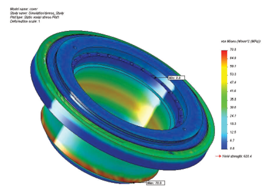
Cover – 20" Class 600 – Fully Welded Type
